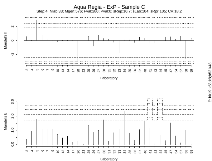
Figure IV.291: Mandel h/k plot - Sample C - Extractable P
