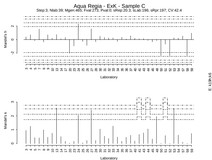
Figure IV.241: Mandel h/k plot - Sample C – Extractable K
