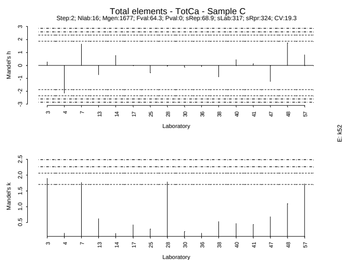
Figure IV.342: Mandel's h/k plot - Sample C – Total Ca
