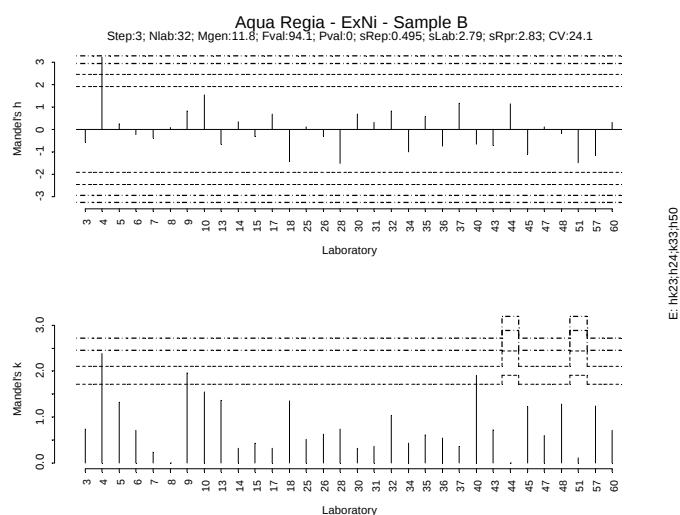
Figure IV.280: Mandel h/k plot - Sample B - Extractable Ni
