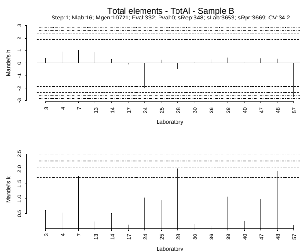
Figure IV.330: Mandel h/k plot - Sample B – Total Al
