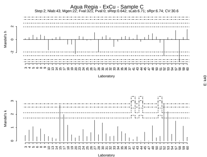
Figure IV.211: Mandel h/k plot - Sample C – Extractable Cu
