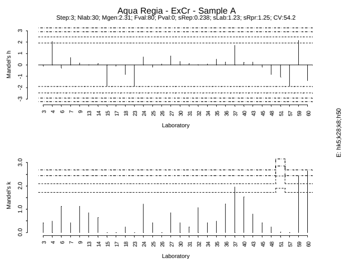
Figure IV.199: Mandel h/k plot - Sample A – Extractable Cr
