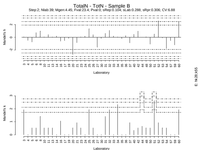
Figure IV. 71: Mandel h/k plot - Sample B – Total N
