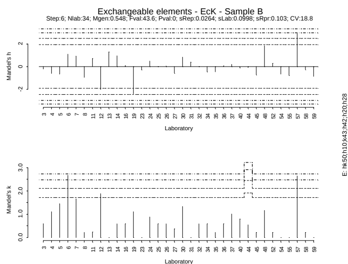
Figure IV.120: Sample B mean – Exchangeable K
