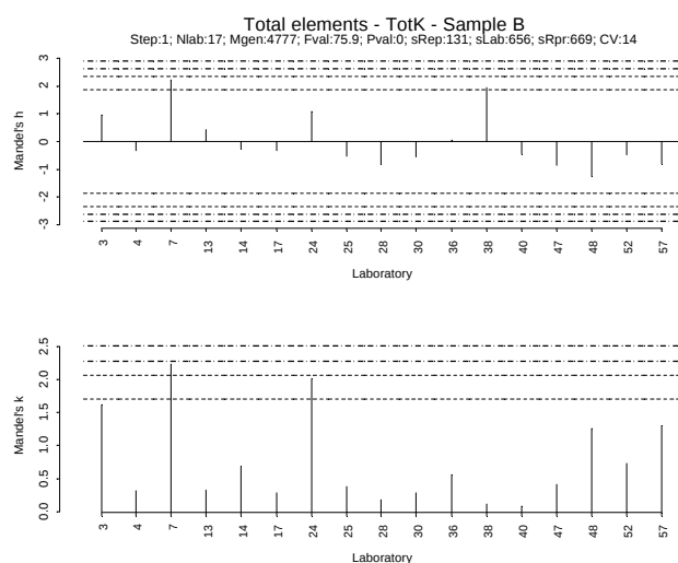
Figure IV.360: Mandel h/k plot - Sample B – Total K
