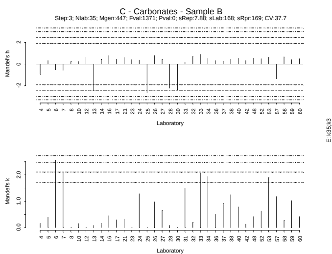
Figure IV. 52: Mandel h/k plot - Sample B mean - Carbonates
