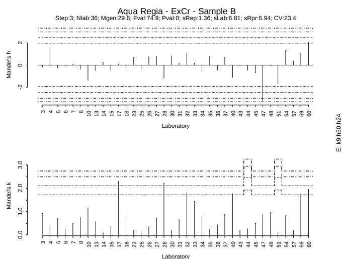
Figure IV.200: Mandel h/k plot - Sample B – Extractable Cr
