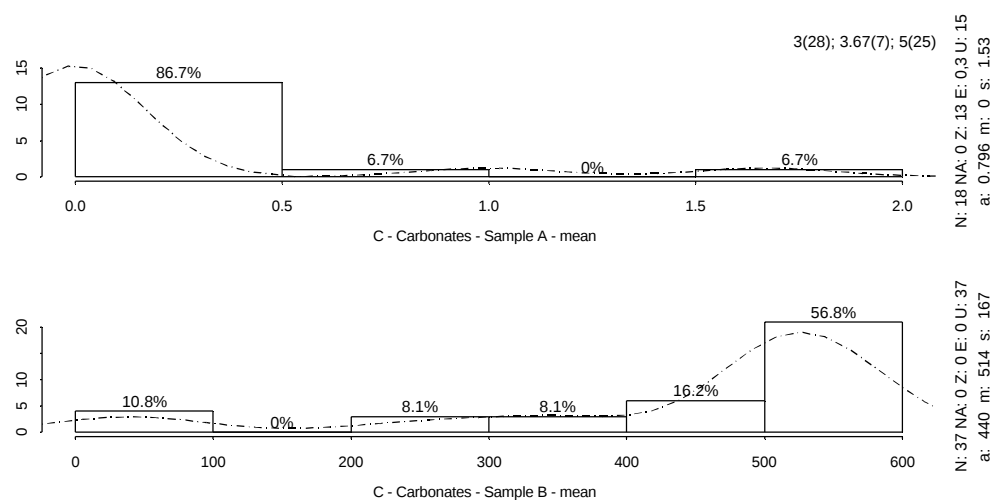
Figure IV. 45: Histogram mean - Carbonates
