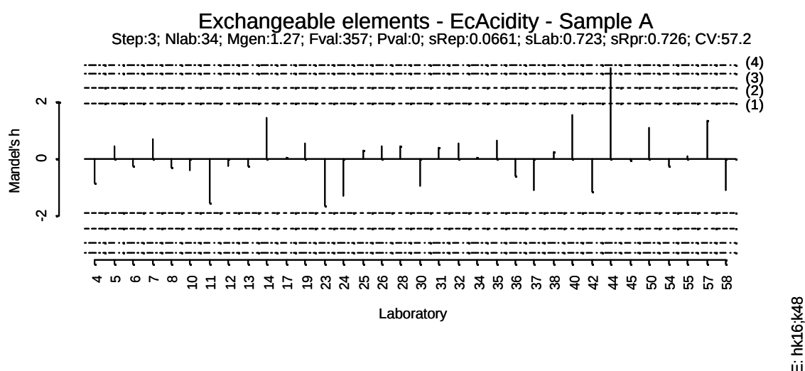
Figure I.7: Mandel's h statistic for sample A for the parameter 'Exchangeable acidity'
