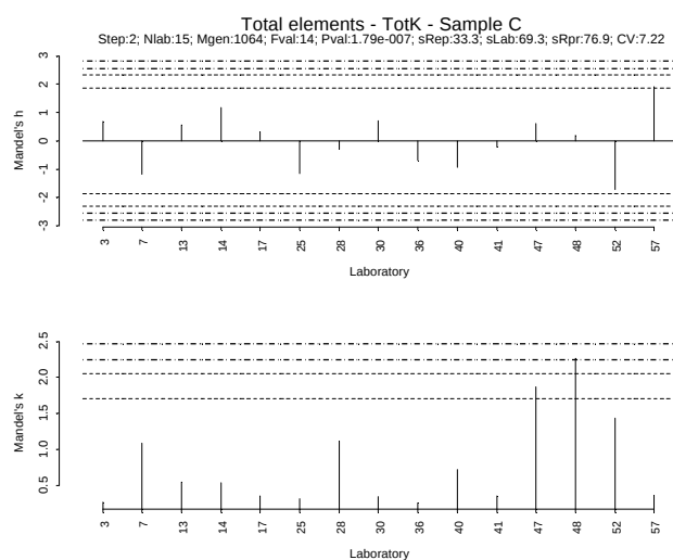
Figure IV.361: Mandel h/k plot - Sample C – Total K
