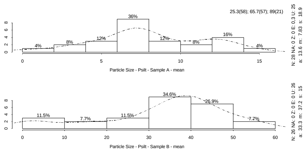
Figure IV. 9: Histogram showing the distribution of the reported mean values of silt
