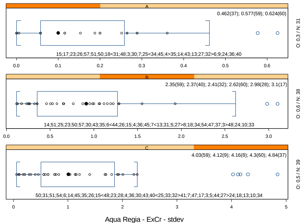
Figure IV.195: Boxplot stdev – Extractable Cr
