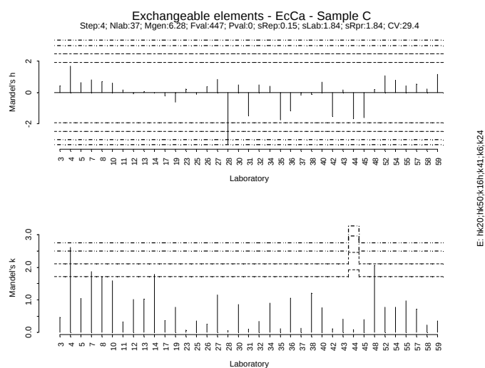
Figure IV. 101: Mandel h/k plot - Sample C mean - Exchangeable Ca
