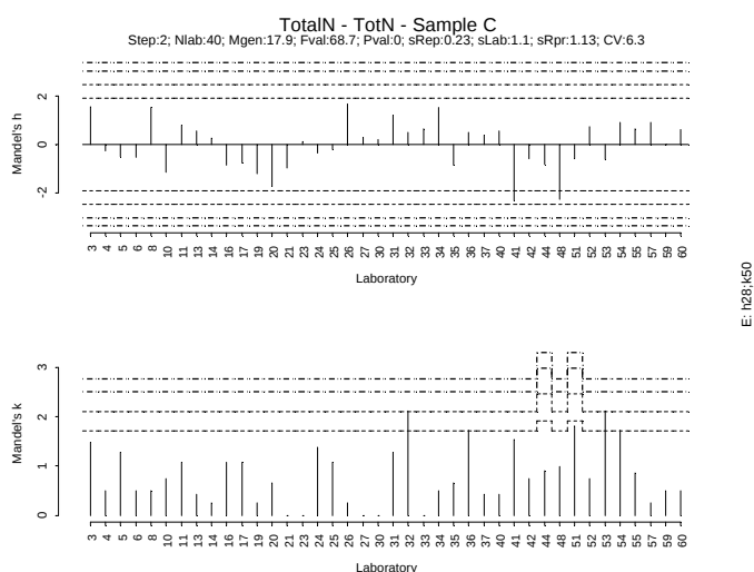
Figure IV. 72: Mandel h/k plot - Sample C – Total N
