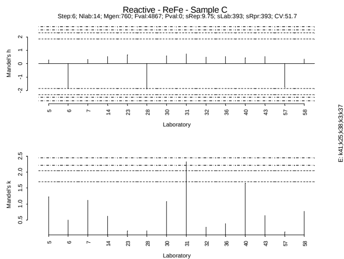
Figure IV.411: Mandel h/k plot - Sample C – Reactive Fe
