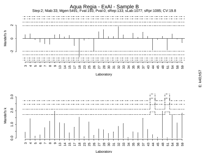
Figure IV.170: Mandel h/k plot - Sample B – Extractable Al
