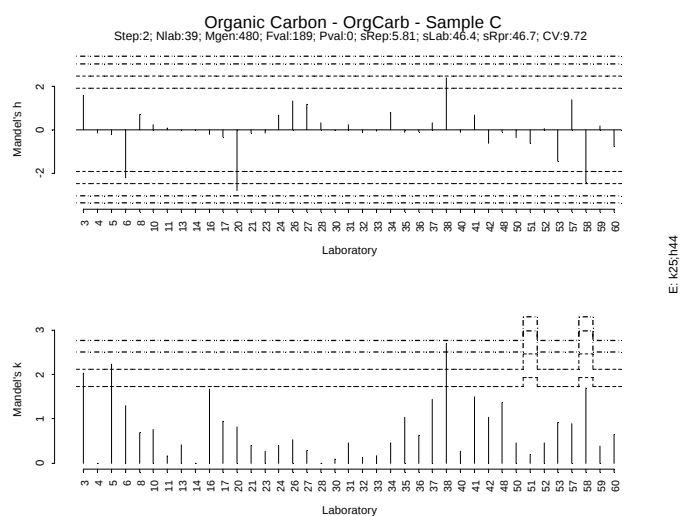
Figure IV. 62: Mandel's h and k plot - Sample C mean – Organic carbon
