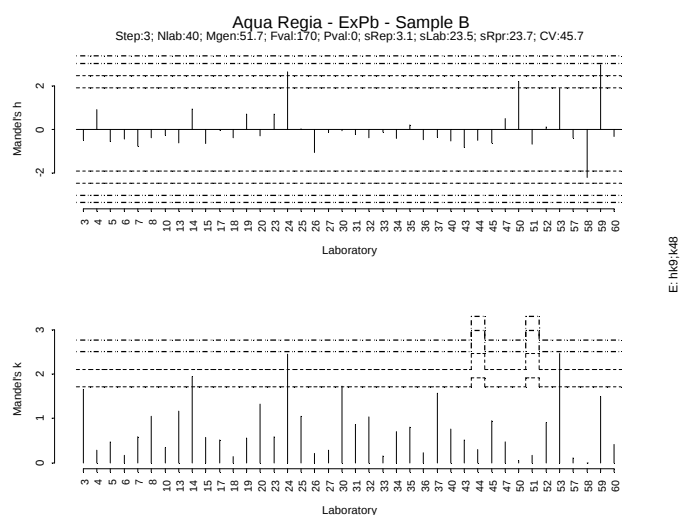
Figure IV.300: Mandel h/k plot - Sample B - Extractable Pb
