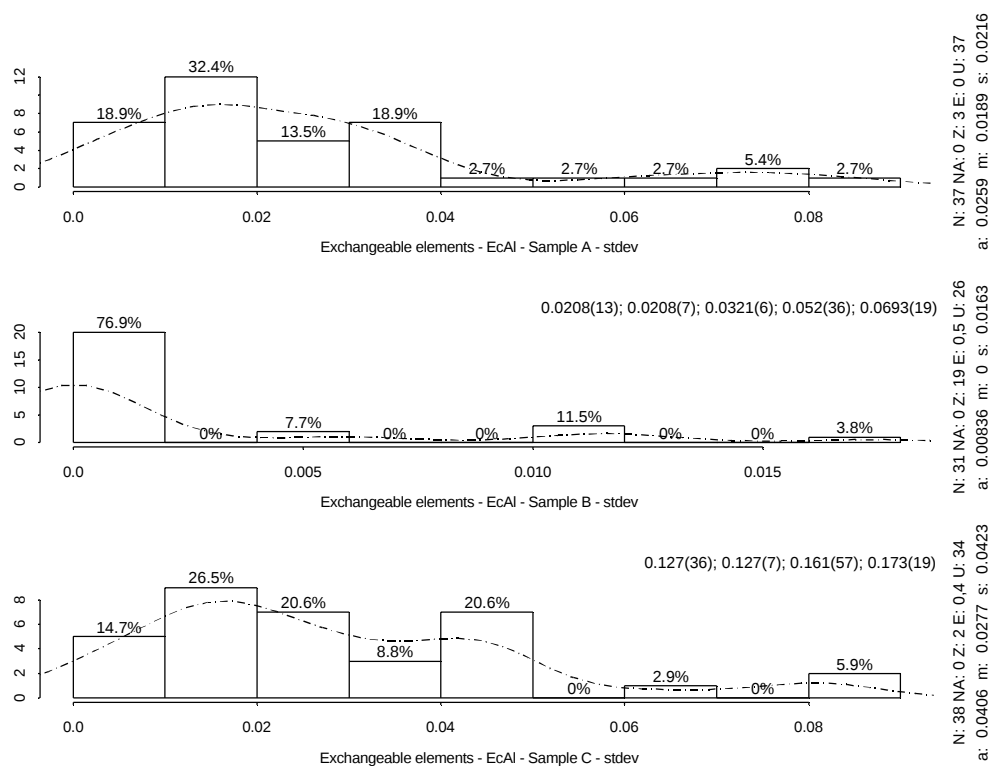
Figure IV. 85: Histogram stdev - Exchangeable AI
