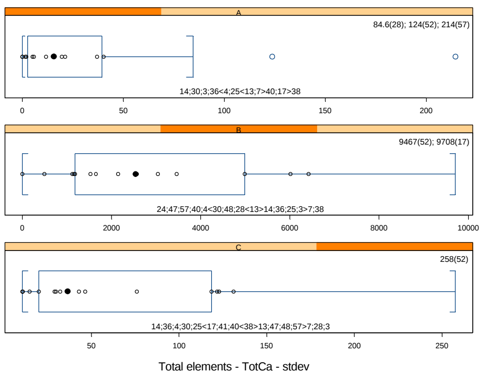
Figure IV.336: Boxplot stdev – Total Ca
