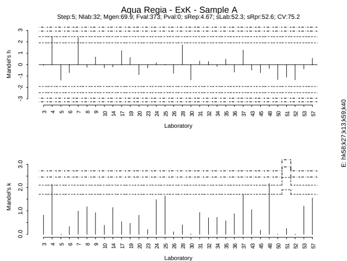
Figure IV.239: Mandel h/k plot - Sample A – Extractable K
