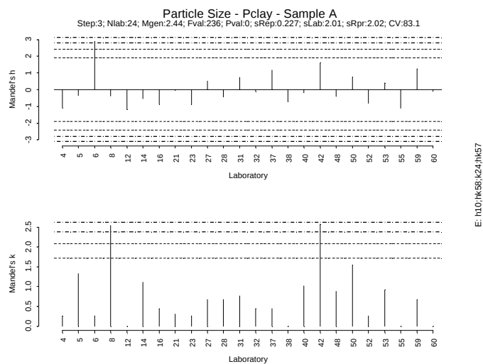
Figure IV.7: Mandel's h and k plot - Sample A – Particle Size Clay
