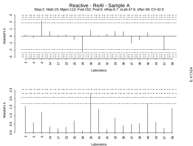
Figure IV.399: Mandel h/k plot - Sample A– Reactive Al
