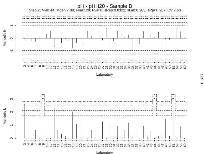
Figure IV.43: Mandel's h and k plot - Sample B - pH(H 2 O)
