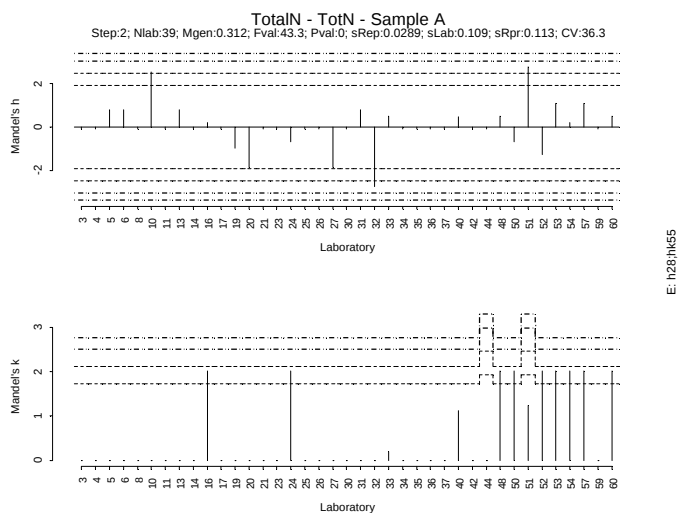
Figure IV. 70: Mandel h/k plot - Sample A – Total N
