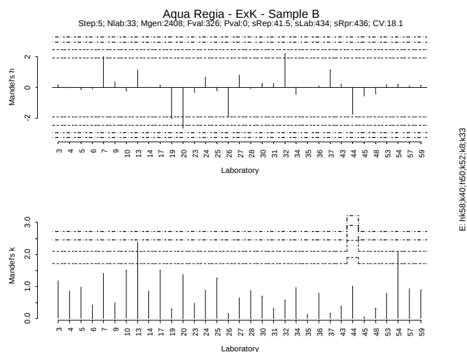
Figure IV.240: Mandel h/k plot - Sample B – Extractable K
