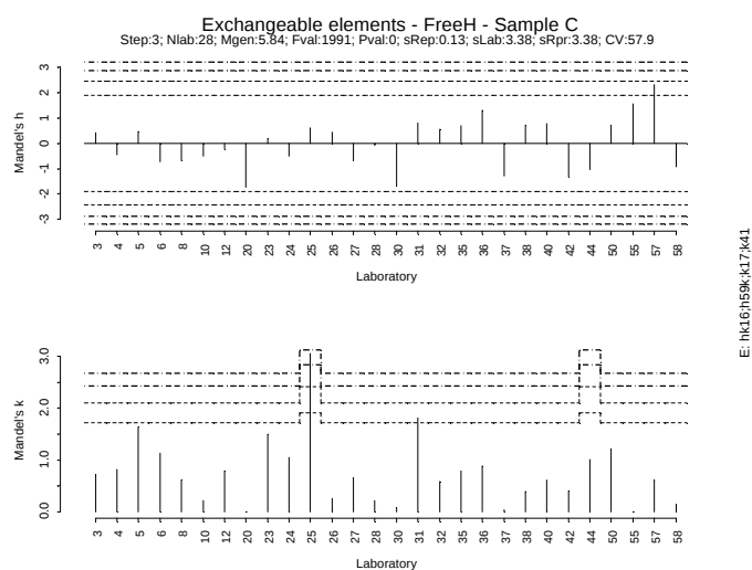
Figure IV.161: Mandel's h and k plot - Sample C - Free H + acidity
