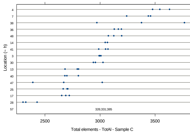
Figure IV.328: Dotplot - Sample C – Total AI
