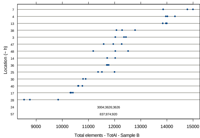
Figure IV.327: Dotplot - Sample B – Total AI
