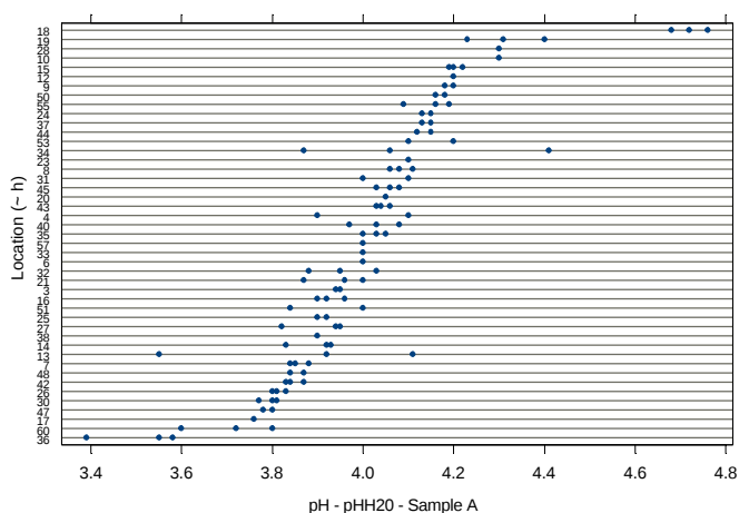
Figure IV.39: Dotplot - Sample A - pH(H 2 O)
