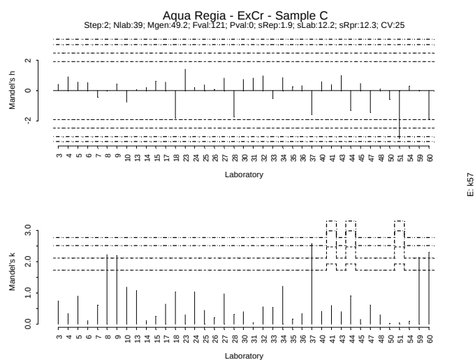
Figure IV.201: Mandel h/k plot - Sample C – Extractable Cr
