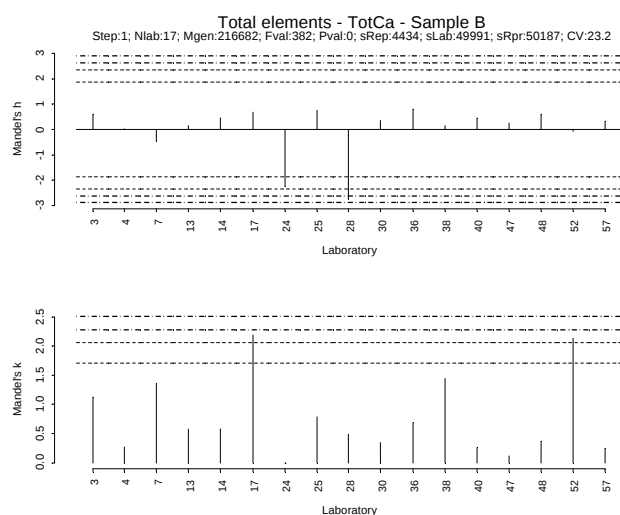
Figure IV.341: Mandel h/k plot - Sample B – Total Ca
