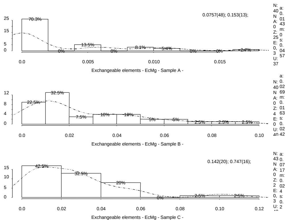
Figure IV.124: Histogram stdev – Exchangeable Mg
