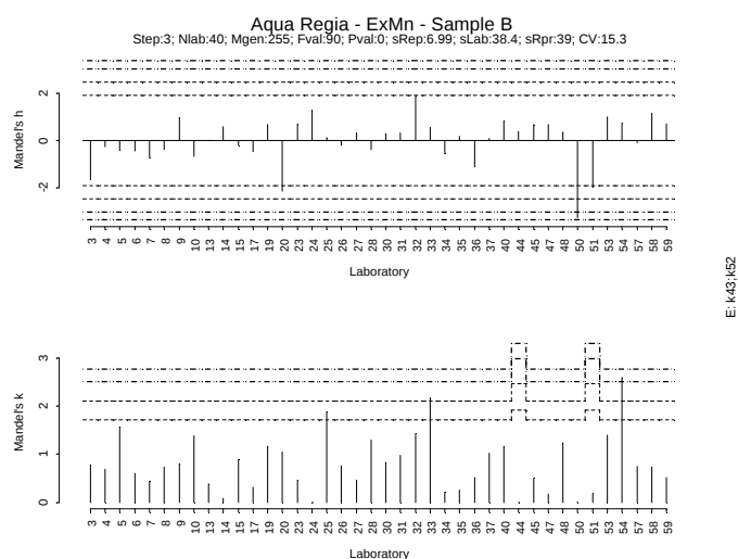
Figure IV.260: Sample B - Extractable Mn
