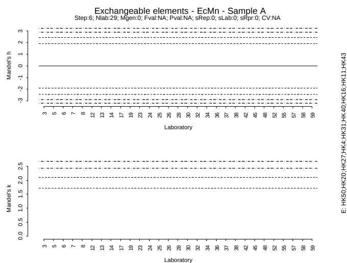
Figure IV.139: Mandel h/k plot - Sample A – Exchangeable Mn
