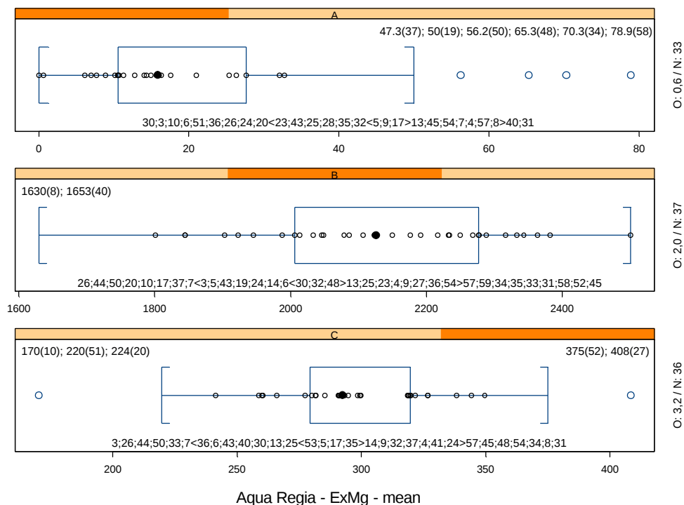
Figure IV.243: Boxplot mean – Extractable Mg
