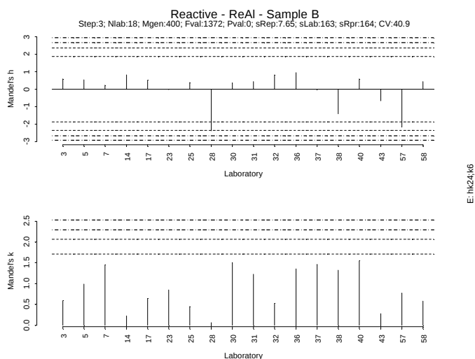
Figure IV.400: Mandel h/k plot - Sample B – Reactive Al
