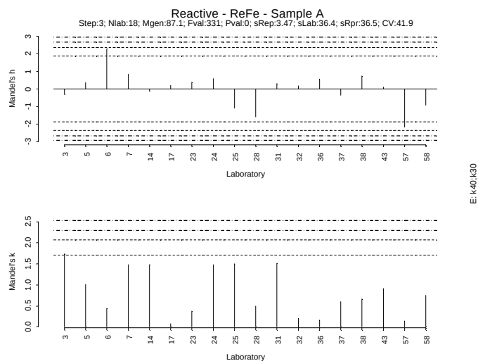
Figure IV.409: Mandel h/k plot - Sample A – Reactive Fe
