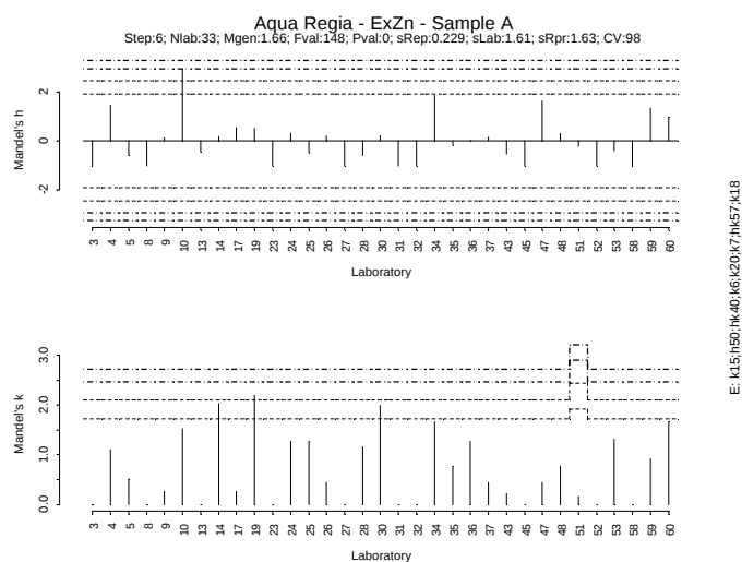
Figure IV. 319: Mandel h/k plot - Sample A - Extractable Zn
