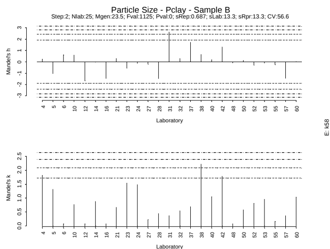
Figure IV.8: Mandel's h and k plot - Sample B – Particle Size Clay
