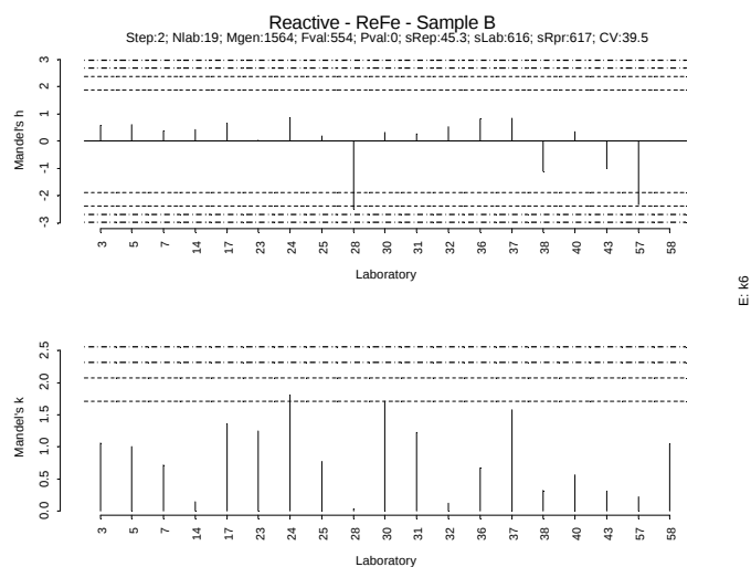
Figure IV.410: Mandel h/k plot - Sample B – Reactive Fe
