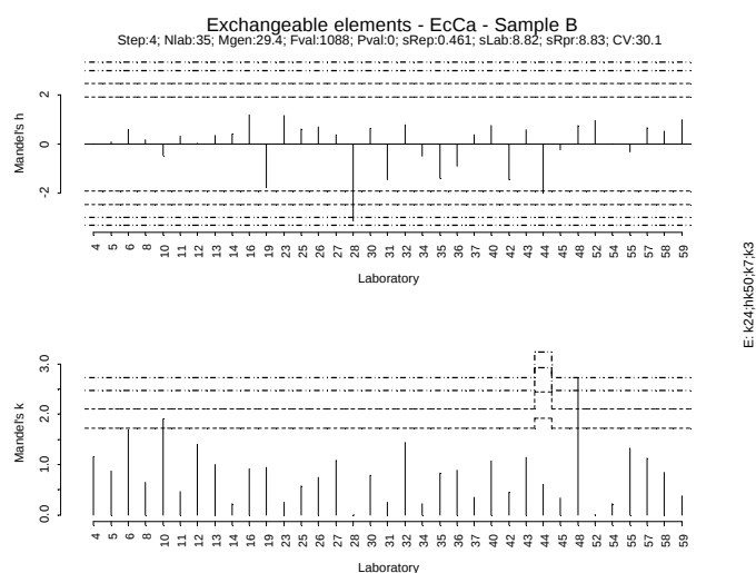
Figure IV. 100: Mandel h/k plot - Sample B mean - Exchangeable Ca
