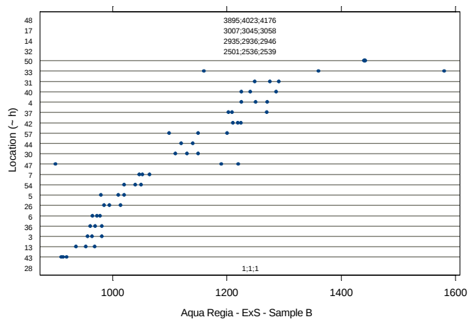
Figure IV.307: Dotplot - Sample B - Extractable S
