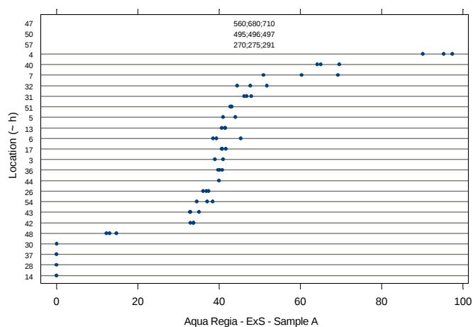
Figure IV.306: Dotplot - Sample A- Extractable S
