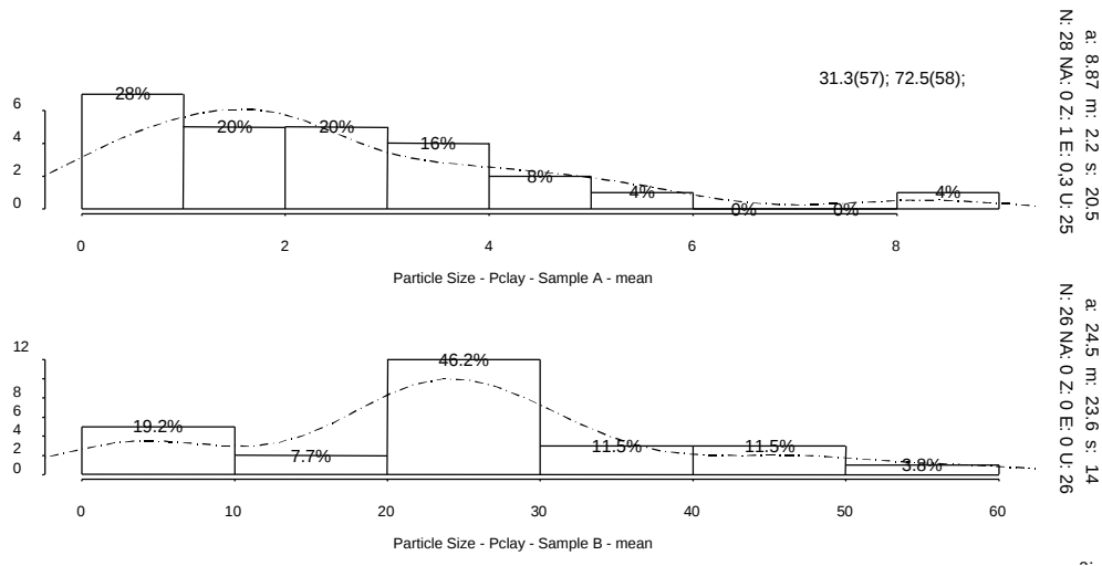
Figure IV. 1: Histogram showing the distribution of the reported mean values of clay
