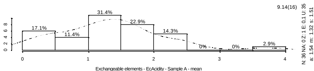
Figure I.2: Histogram showing relative percentages and a rescaled density curve of the mean of 3 replicates of the measured parameter 'exchangeable acidity' on Sample A. The units of the x-axis are in \text{cmol}(+)/\text{kg} .
