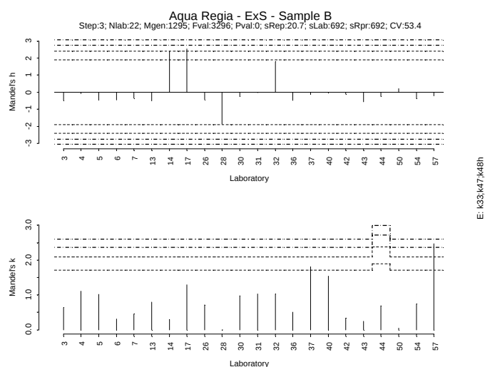
Figure IV.310: Mandel h/k plot - Sample B - Extractable S
