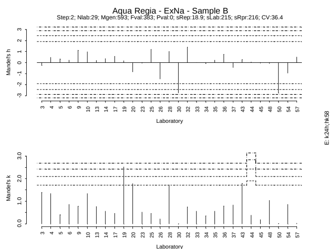
Figure IV.270: Mandel h/k plot - Sample B - Extractable Na
