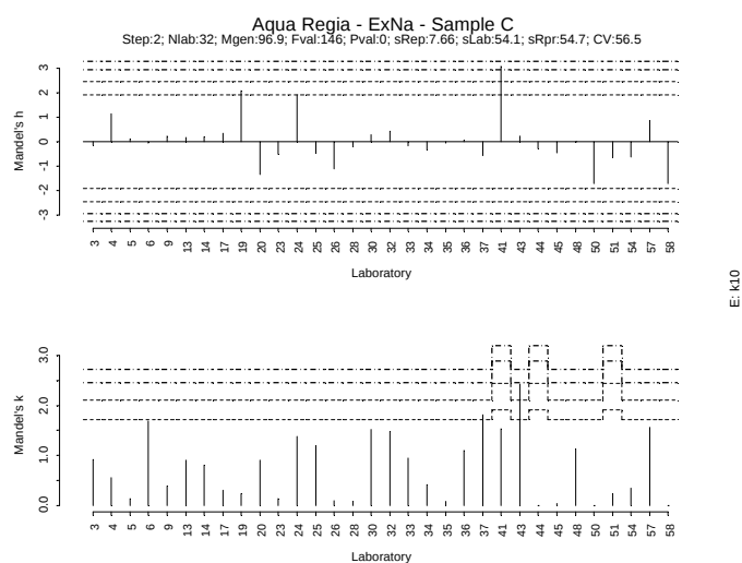
Figure IV.271: Mandel h/k plot - Sample C - Extractable Na
