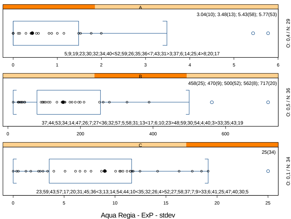
Figure IV.285: Boxplot stddev - Extractable P
