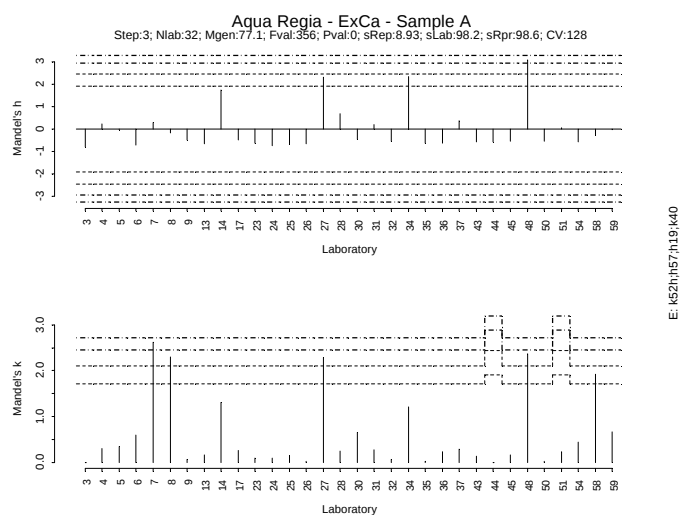
Figure IV.179: Mandel h/k plot - Sample A – Extractable Ca
