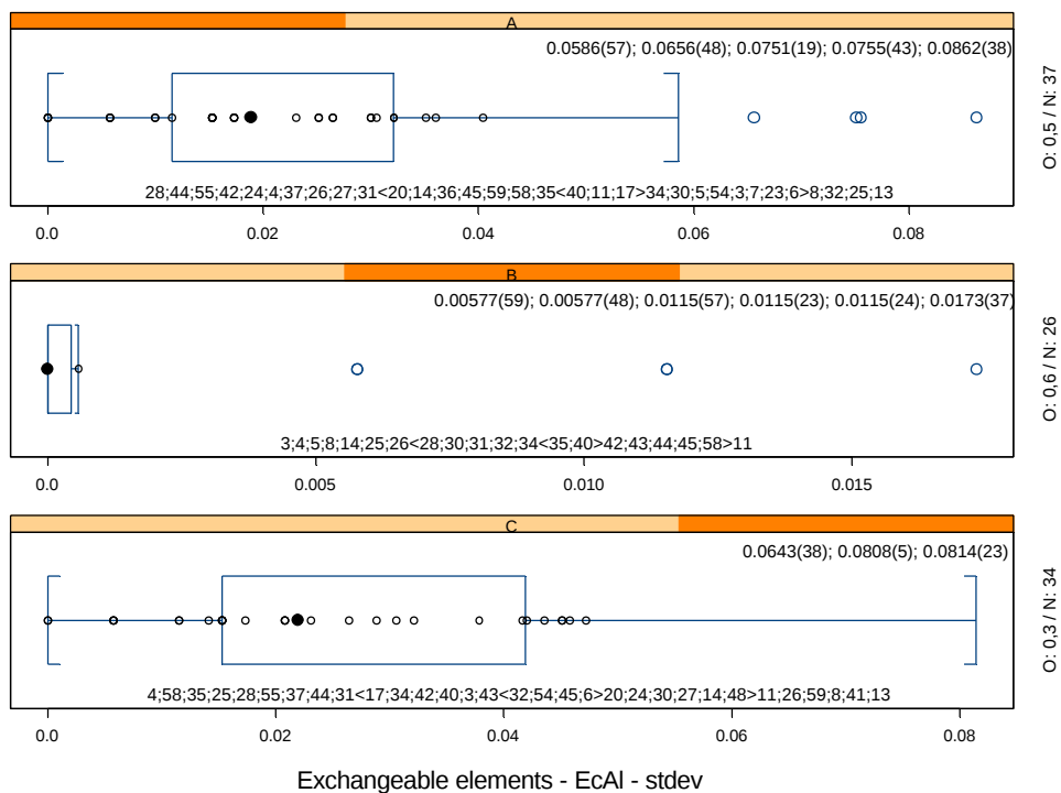
Figure IV. 86: Boxplot stdev - Exchangeable AI
