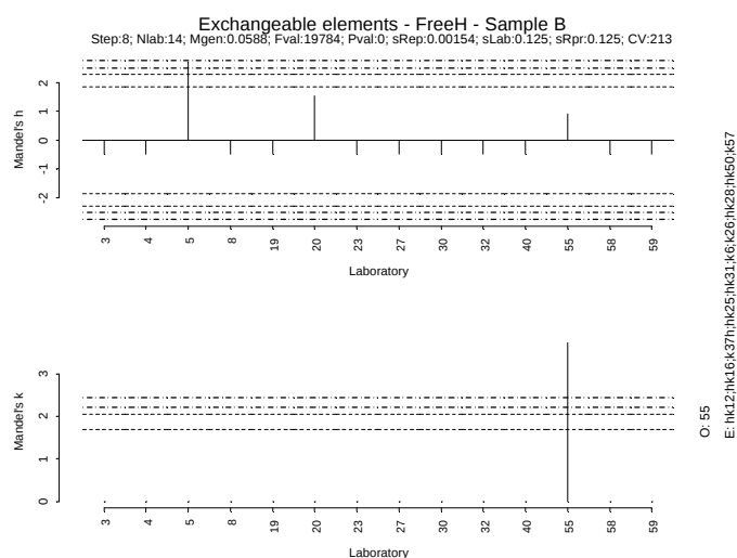
Figure IV.160: Mandel's h and k plot - Sample B - Free H + acidity
