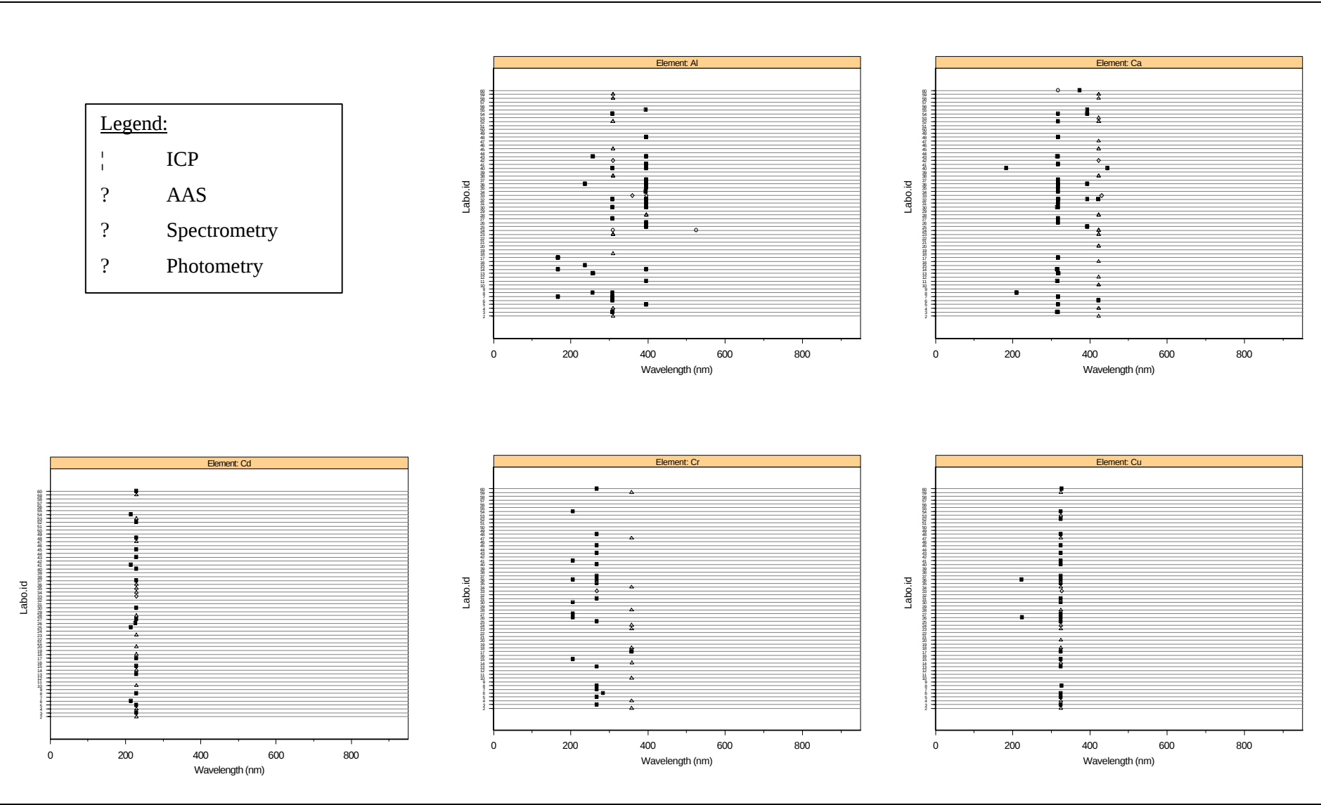
Figure VIII.1: Dotplots – Wavelengths used for the analysed elements
