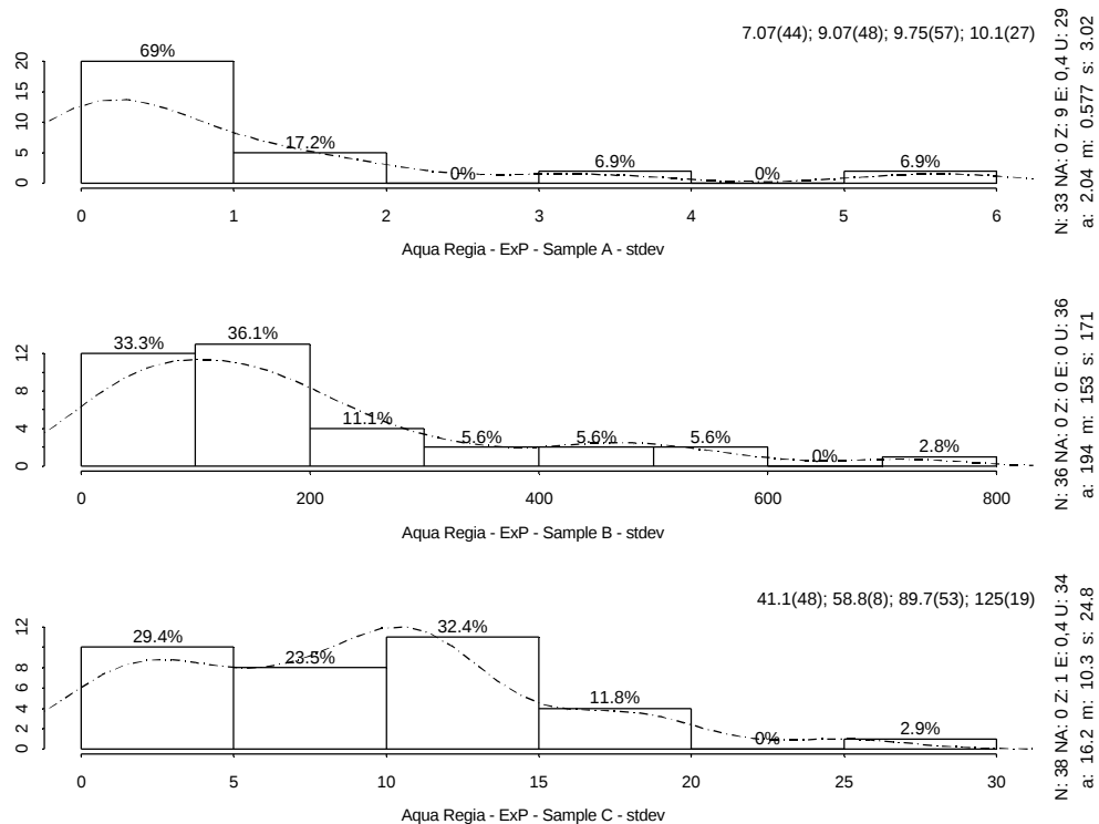
Figure IV.284: Histogram stddev - Extractable P
