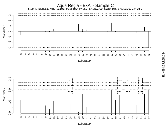
Figure IV.171: Mandel h/k plot - Sample C – Extractable Al
