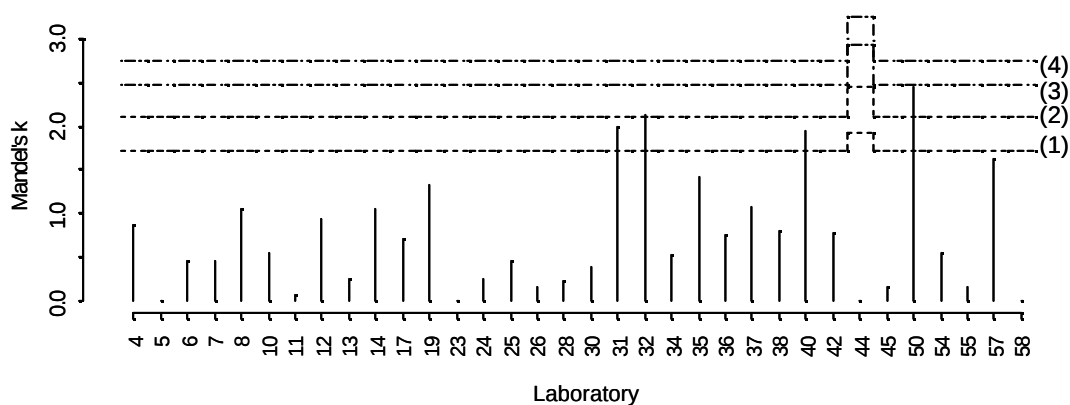
Figure I.8: Mandel's k statistics for sample A for the parameter 'Exchangeable acidity'
