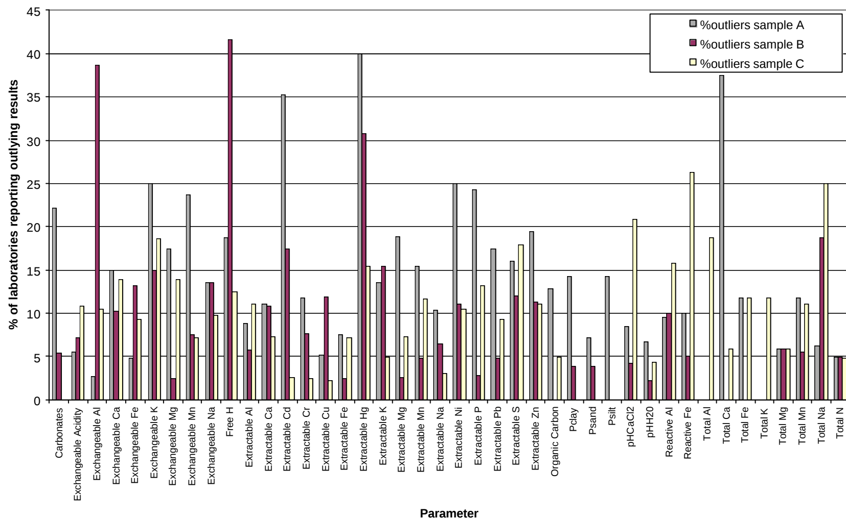
Figure I.17: % of number of laboratories, which participated for that particular parameter, reporting outlying results (probability level 99%)
