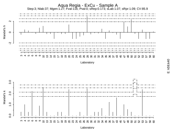
Figure IV.209: Mandel h/k plot - Sample A – Extractable Cu
