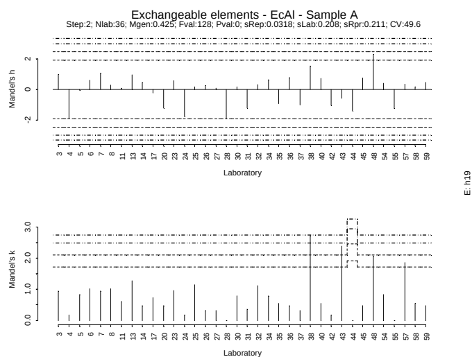
Figure IV. 89: Mandel h/k plot - Sample A - Exchangeable Al
