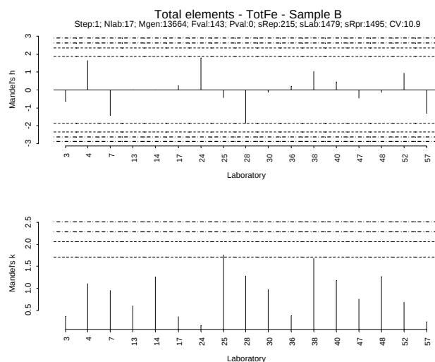
Figure IV.350: Mandel h/k plot - Sample B – Total Fe
