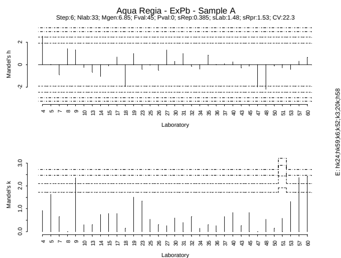
Figure IV.299: Mandel h/k plot - Sample A - Extractable Pb
