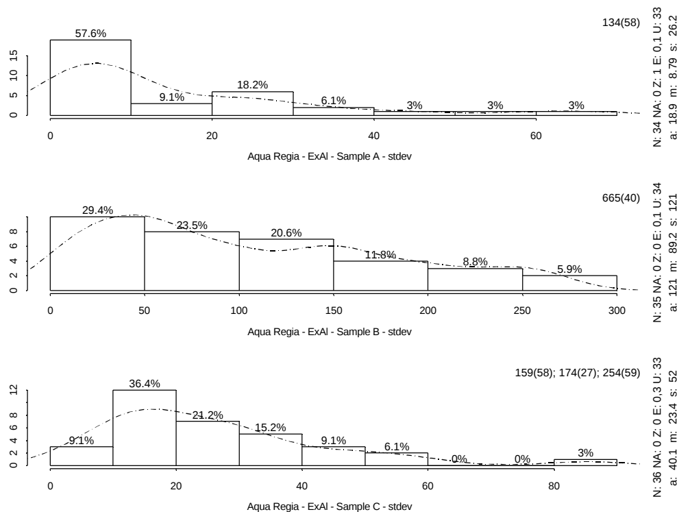
Figure IV.164: Histogram stdev – Extractable AI
