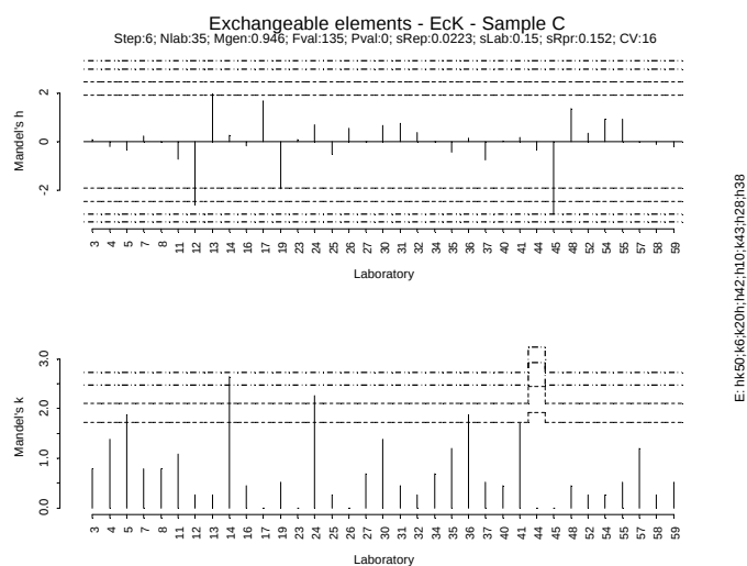
Figure IV.121: Sample C mean – Exchangeable K
