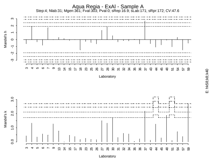
Figure IV.169: Mandel h/k plot - Sample A – Extractable Al
