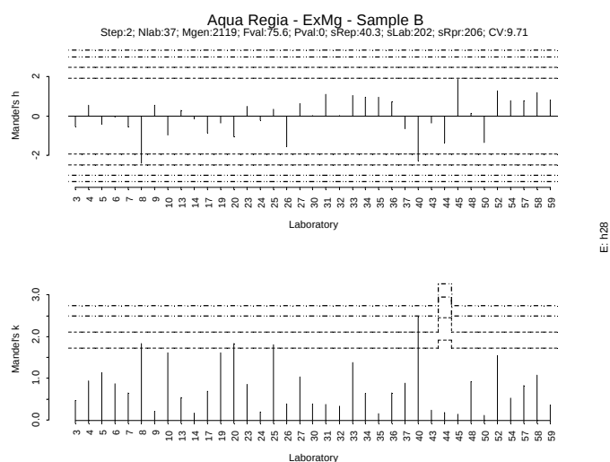
Figure IV.250: Mandel h/k plot - Sample B – Extractable Mg
