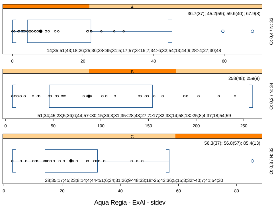
Figure IV.165: Boxplot stdev – Extractable AI
