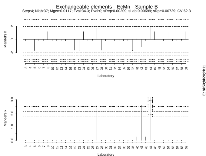
Figure IV.140: Mandel h/k plot - Sample B – Exchangeable Mn
