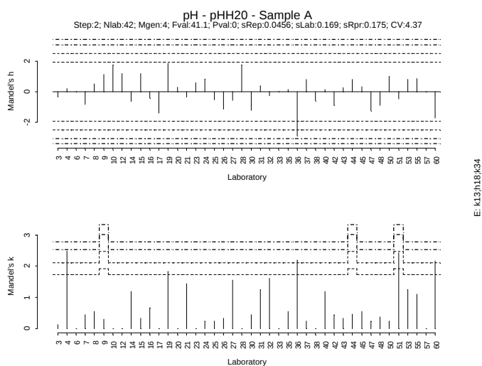
Figure IV.42: Mandel's h and k plot - Sample A - pH(H 2 O)
