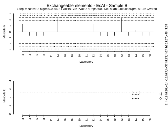
Figure IV. 90: Mandel h/k plot - Sample B - Exchangeable Al
