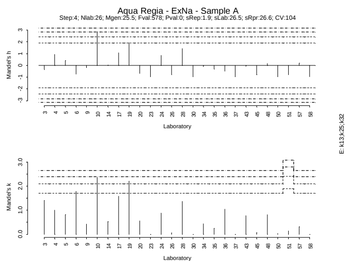
Figure IV.269: Mandel h/k plot - Sample A - Extractable Na
