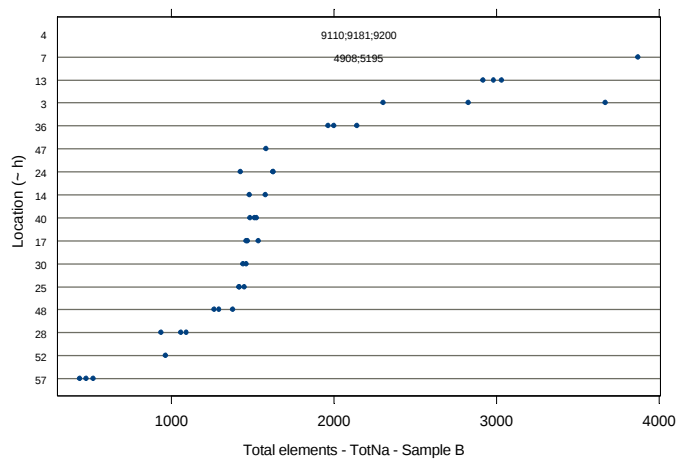
Figure IV.387: Dotplot - Sample B – Total Na
