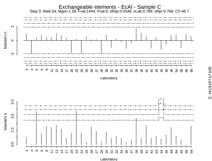
Figure IV. 91: Mandel h/k plot - Sample C - Exchangeable Al
