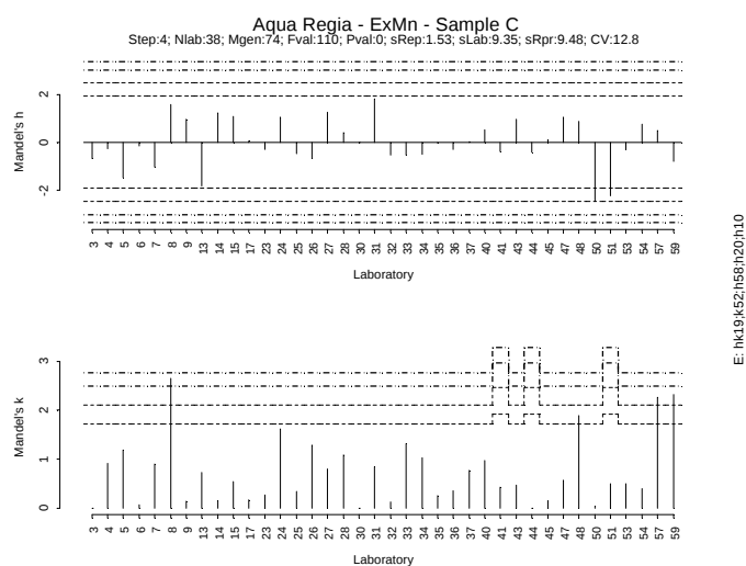
Figure IV.261: Sample Cv - Extractable Mn
