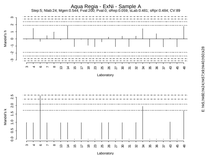
Figure IV.279: Mandel h/k plot - Sample A - Extractable Ni
