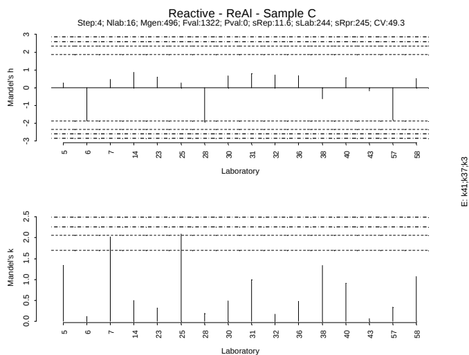
Figure IV.401: Mandel h/k plot - Sample C – Reactive Al
