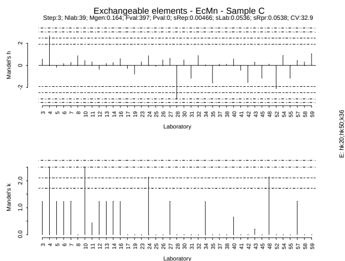
Figure IV.141: Mandel h/k plot - Sample C – Exchangeable Mn
