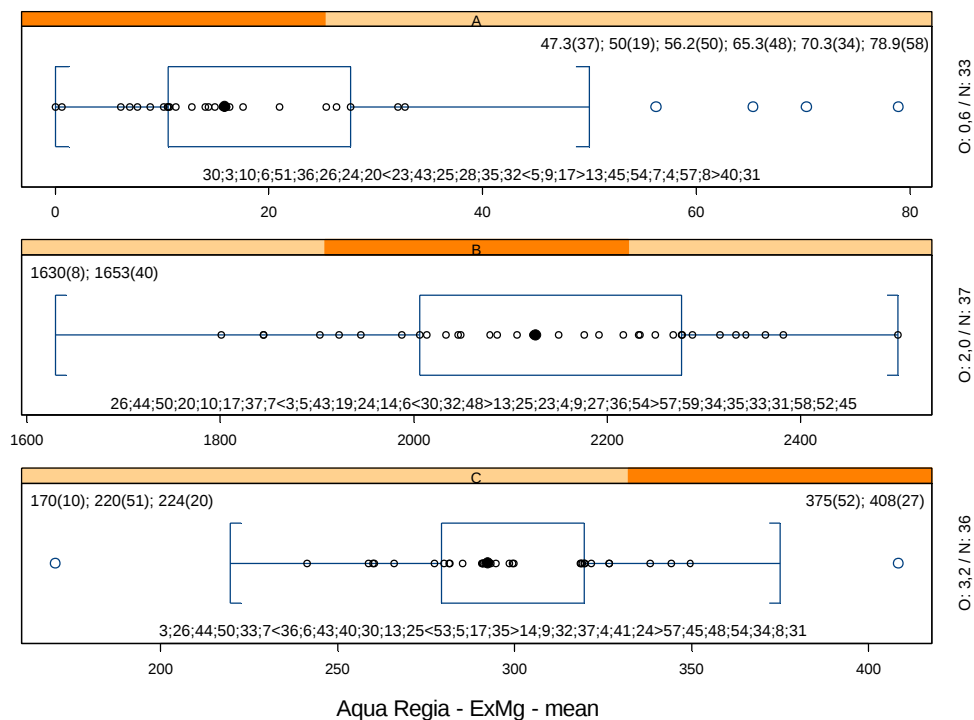
Figure IV.123: Boxplot mean – Exchangeable Mg
