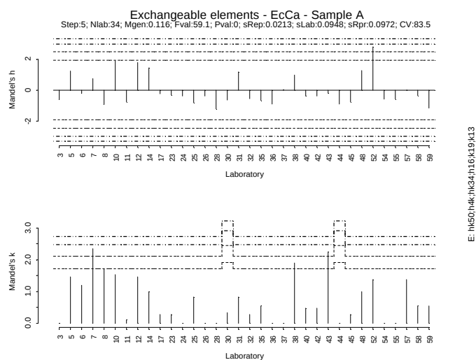
Figure IV. 99: Mandel h/k plot - Sample A - Exchangeable Ca
