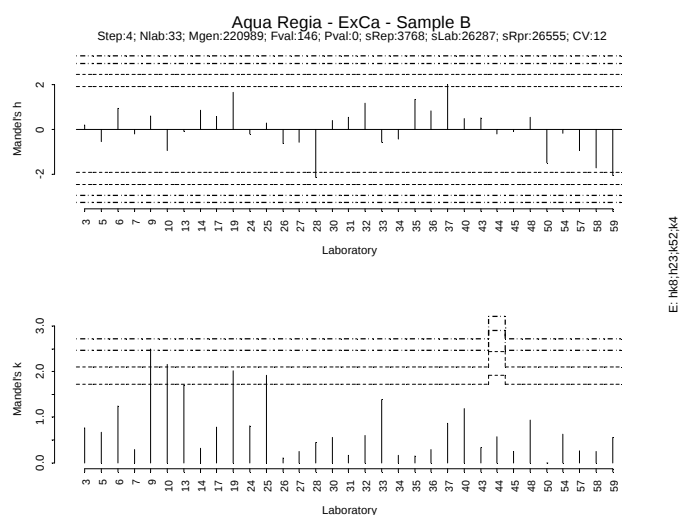
Figure IV.180: Mandel h/k plot - Sample B – Extractable Ca
