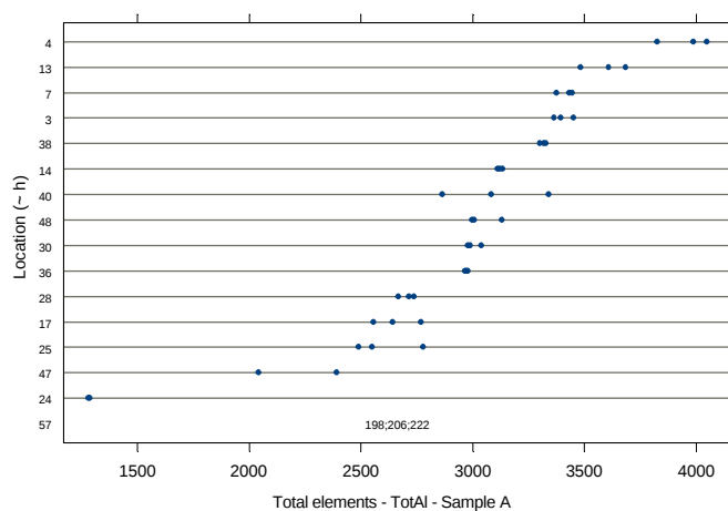
Figure IV.326: Dotplot - Sample A – Total AI
