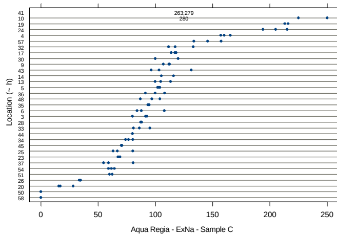
Figure IV.268: Dotplot - Sample C - Extractable Na
