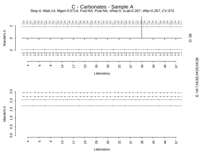
Figure IV. 51: Mandel h/k plot - Sample A - Carbonates
