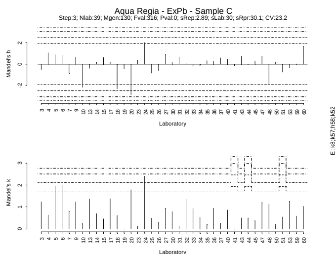
Figure IV.301: Mandel h/k plot - Sample C - Extractable Pb
