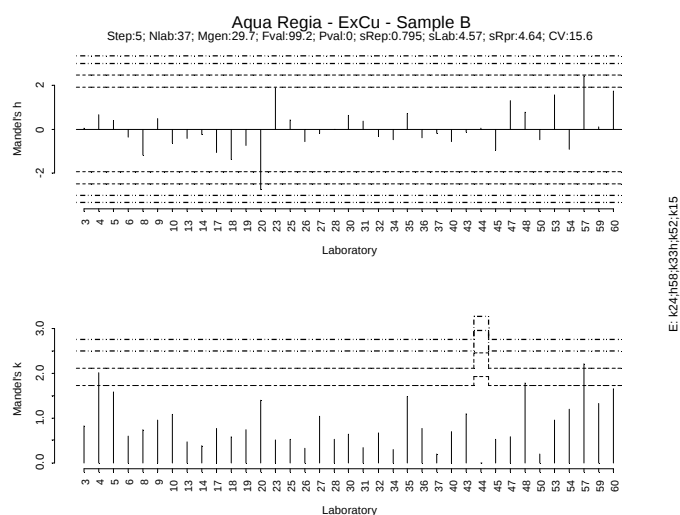
Figure IV.210: Mandel h/k plot - Sample B – Extractable Cu
